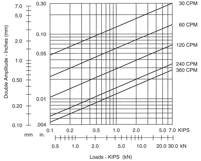
Force-Frequency-Amplitude Data
