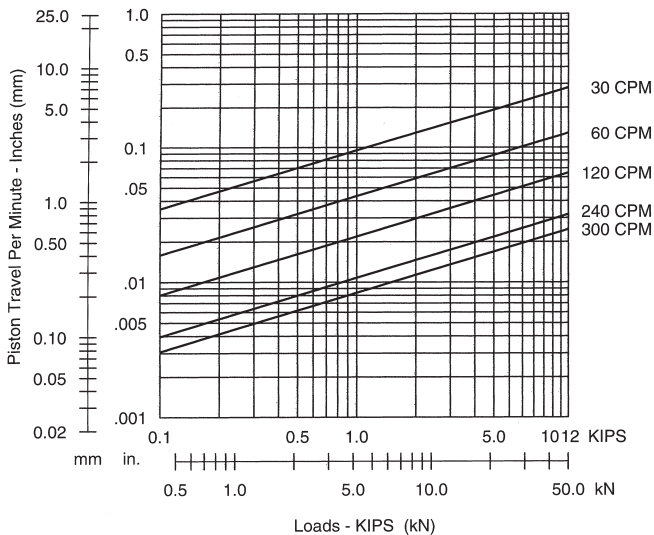
Force-Frequency-Amplitude Data
